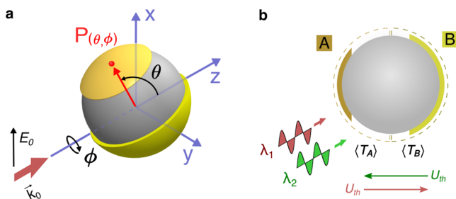
Figure 1. Light beam impinges on an asymmetric particle consisting of a uniform dielectric core and two opposing caps, labeled A and B. The caps are made of materials that allow for selective light absorption based on the wavelength of the incident beam ( \lambda_1 , red; \lambda_2 , green). As a result, the direction of the temperature gradient ( \langle T_A \rangle - \langle T_B \rangle ) is wavelength-dependent. The optically induced thermophoretic drift U_{th} , proportional to the temperature gradient, can be used to transport the particle in space (the guiding scheme is illustrated in Figure 4). (a) 3D view and (b) cross-section of a polystyrene particle with a titanium-nitride (A) and gold (B) cap.
